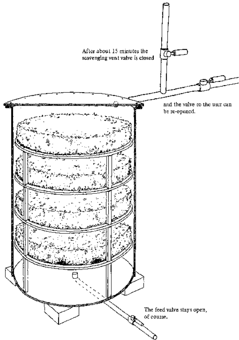
Abbildung 9: Starting up the chamber after refilling with regenerated absorbent (2)
