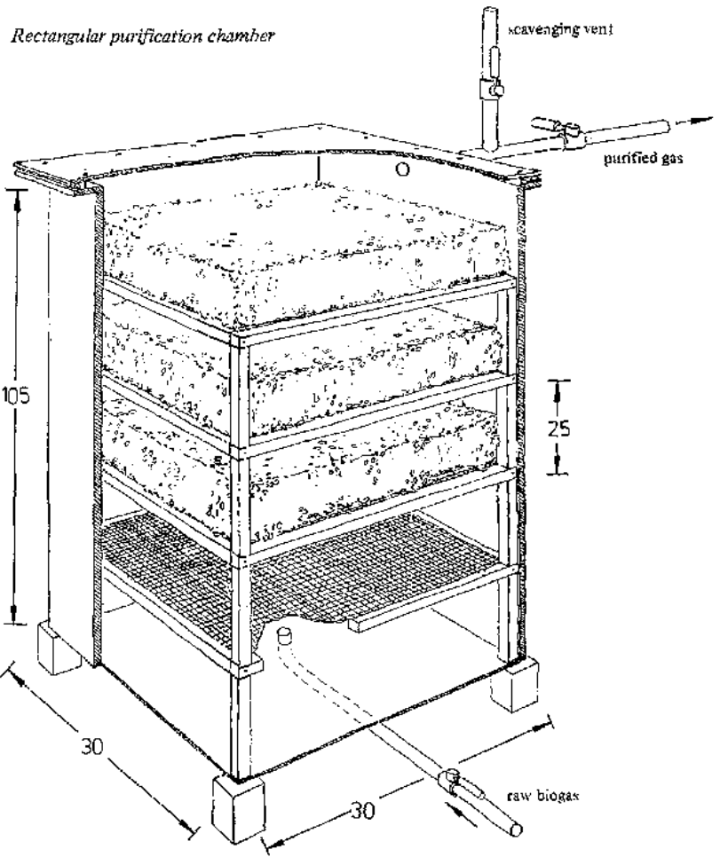
Abbildung 4: Rectangular purification chamber
