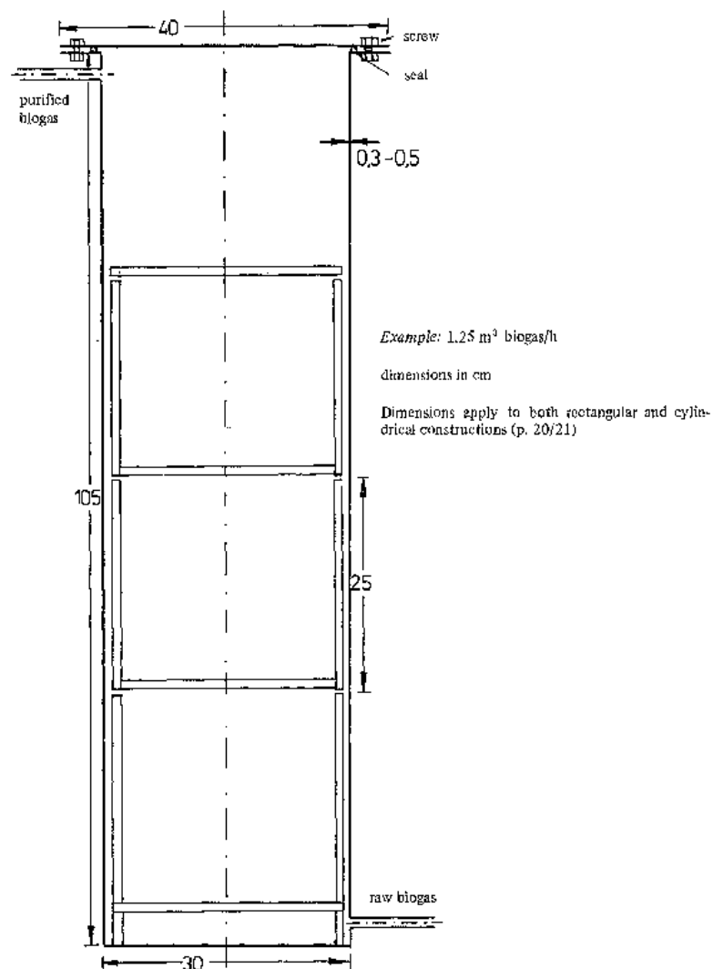
Abbildung 2: Desulphurization chamber for biogas
